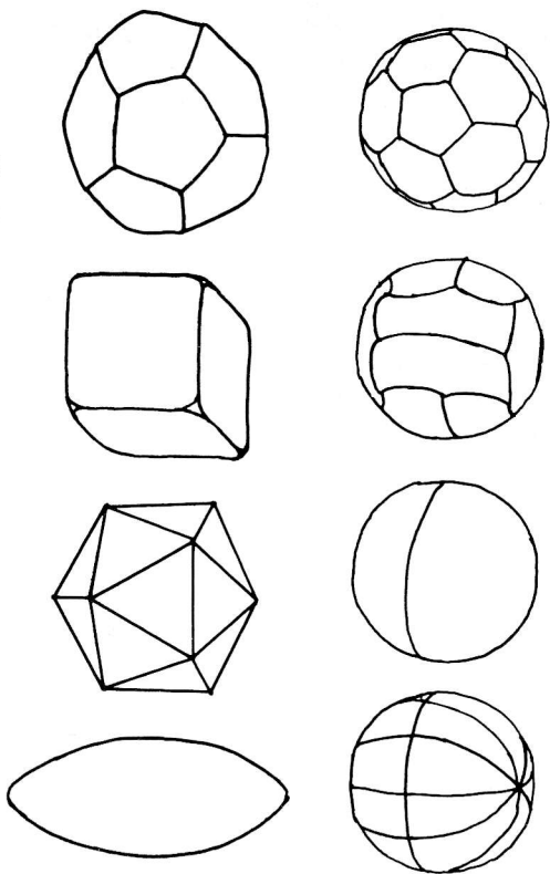
Fig. 23. Some variants of the form of the football.
