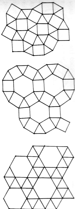
Fig. 20. Examples of plane Archimedean tessellations.
