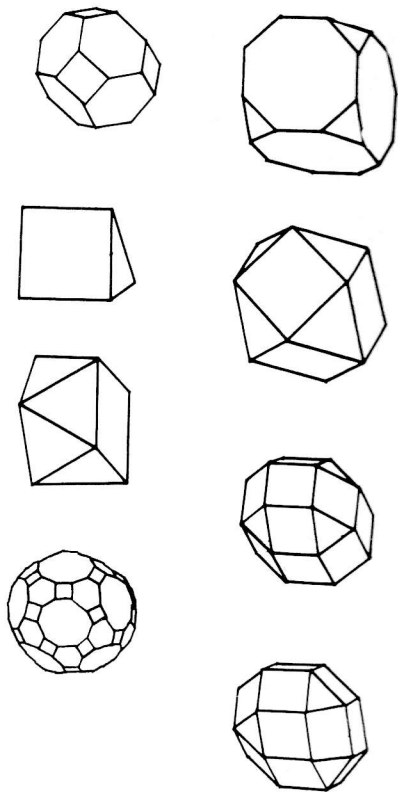
Fig. 22. Pictures of some Archimedean solids.
